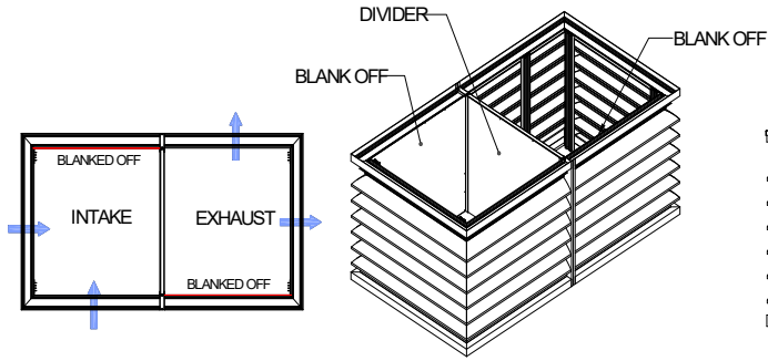
DIVIDER / BAFFLE
